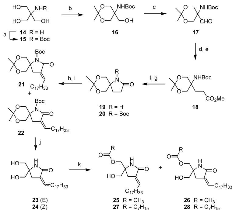
Scheme 3. Reagents and conditions: (a) \text{Boc}_2\text{O} , \text{NEt}_3 , \text{MeOH} ; (b) p\text{-TsOH} , acetone; (c) \text{PCC} , 4 Å mol. sieve, \text{CH}_2\text{Cl}_2 ; (d) \text{PPh}_3\text{CHCO}_2\text{CH}_3 , \text{CH}_2\text{Cl}_2 ; (e) \text{H}_2 , \text{Pd/C} , \text{EtOAc} ; (f) \text{NaOCH}_3 , \text{MeOH} ; (g) \text{Boc}_2\text{O} , \text{NEt}_3 , \text{DMAP} , \text{THF} ; (h) \text{LiHMDS} , \text{THF} ; \text{C}_{17}\text{H}_{33}\text{CHO} ; (i) \text{MsCl} , \text{NEt}_3 , \text{CH}_2\text{Cl}_2 ; \text{DBU} (j) \text{CF}_3\text{CO}_2\text{H} , \text{THF-H}_2\text{O} ; (k) \text{CH}_3\text{COCl} (or \text{C}_7\text{H}_{15}\text{COCl} ), pyridine, \text{CH}_2\text{Cl}_2 .
